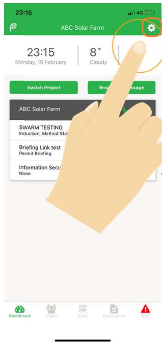
Select Settings
